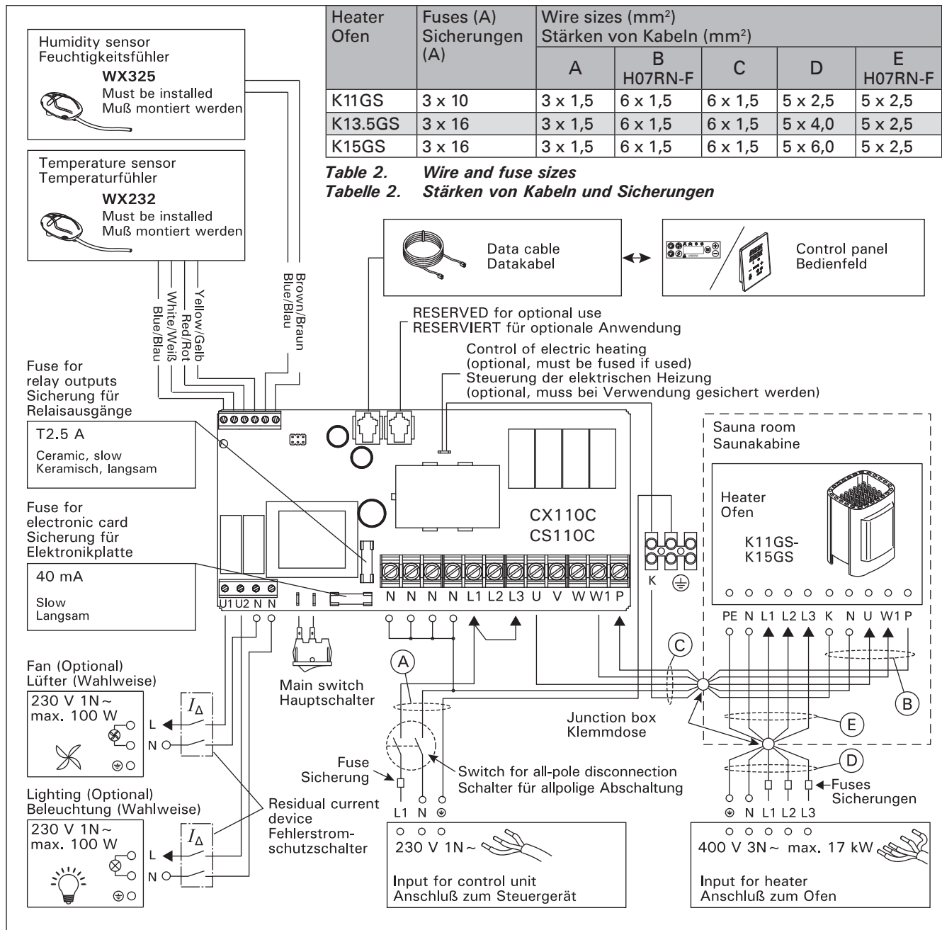
Figure 4. Electrical connections (K11GS–K15GS)
